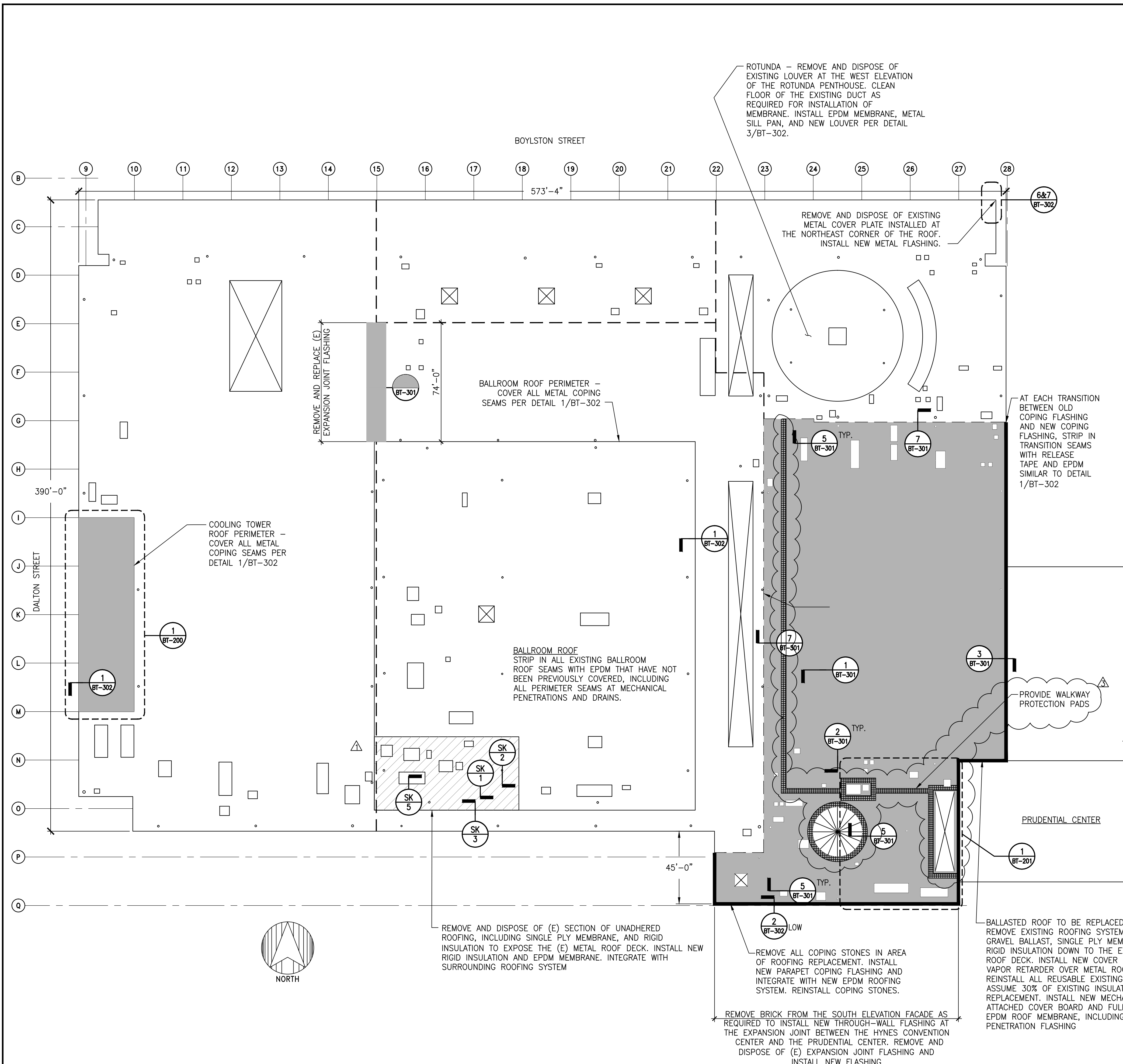
ROOF PLAN SCALE: 1/32" = 1'-0"
